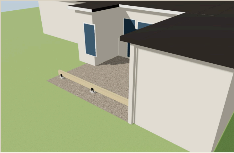
Step 4 · Beams — DROP 6x12 DF S+A (3 posts)
