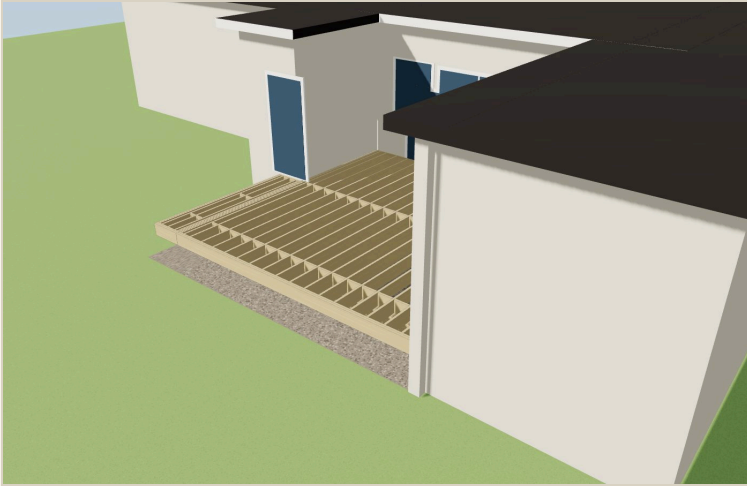
Step 5 · Frame — 2x10 joists at 12", rims, ledger, blocking over the beam
